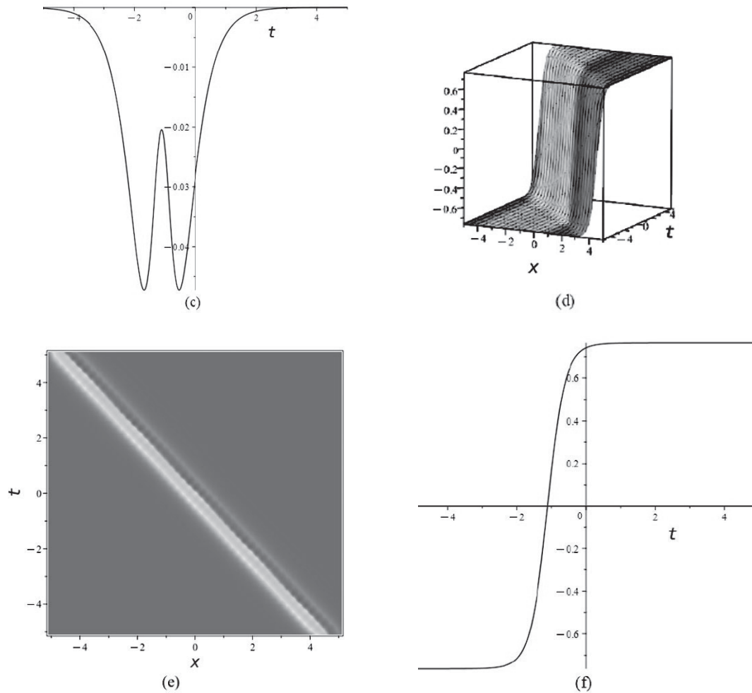
Fig1: The graphical representation of Eq.(3.5): (a) real 3D shape, (b) real density plot, (c) real 2D shape, (d) complex 3D shape, (e) complex density plot and (f) complex 2D shape.
