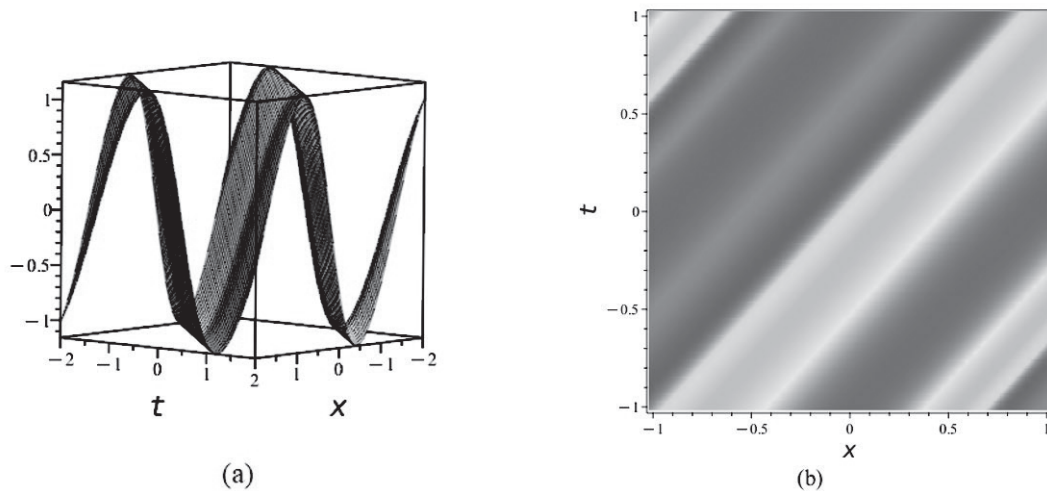
Fig 2: The graphical illustration of Eq. (3.4): (a) real 3D profile, (b) real density plot, (c) real 2D profile, (d) imaginary 3D shape, (e) imaginary density plot and (f) imaginary 2D shape.
