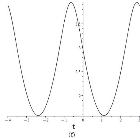
Fig 3: The graphical depiction of Eq. (3.7): (a) real 3D form, (b) real density plot, (c) real 2D shape, (d) complex 3D form, (e) complex density plot and (f) complex 2D shape.
