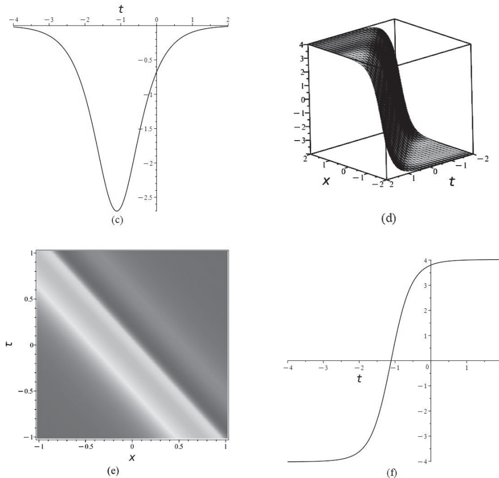
Fig 4: The graphical picture of Eq. (3.5): (a) real 3D nature, (b) real density plot, (c) real 2D nature, (d) complex 3D nature, (e) complex density plot and (f) complex 2D nature .
