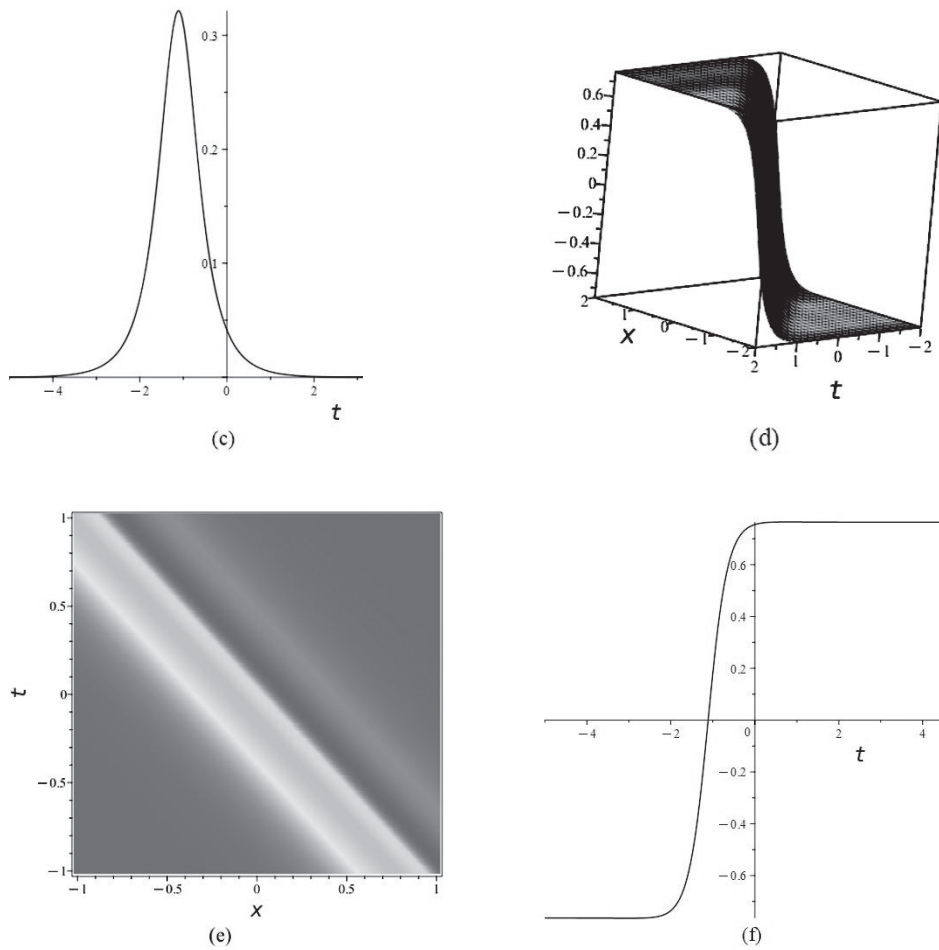
Fig 2: The graphical illustration of Eq. (3.4): (a) real 3D profile, (b) real density plot, (c) real 2D profile, (d) imaginary 3D shape, (e) imaginary density plot and (f) imaginary 2D shape.
